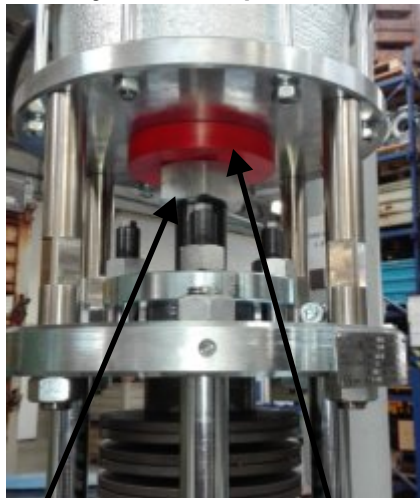
Location of gag iron during the hydro- static pressure test
