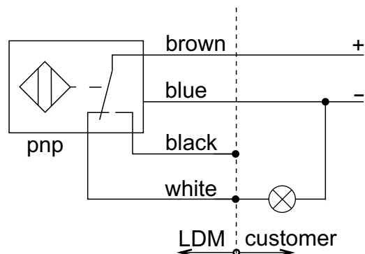
Inductive sensor – wiring diagram:
